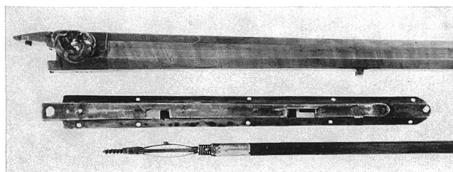
8. Nr 1820. Pipans låsanordning, regelhuset fastskruvat i pipnoten med undre delen gående ner i laddstocksnoten. — The locking-device of the barrel. The bolt-house is fixed in the bottom of the barrel notch with the lower part intruding into the ramrod notch.
